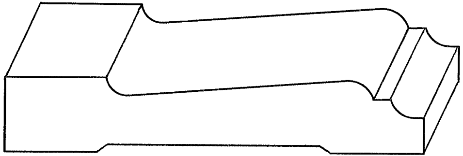
1214 13/16 x 4-1/2
