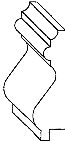
22-8 3/4 x 2-1/2
