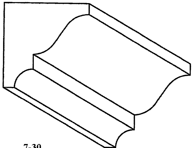
7-30 1-7/16 x 1-7/16
