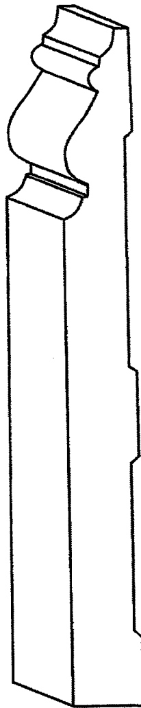
1336 9/16 x 5-1/4
