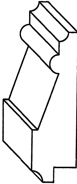
22-11 3/4 x 2-1/2
