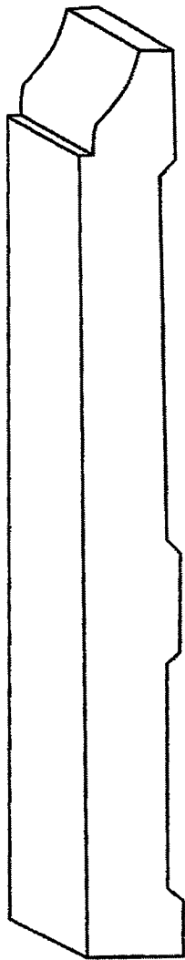
1306 9/16 x 5-1/4
